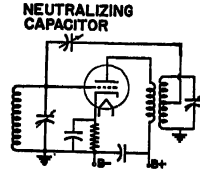
Neurodyne circuit.
